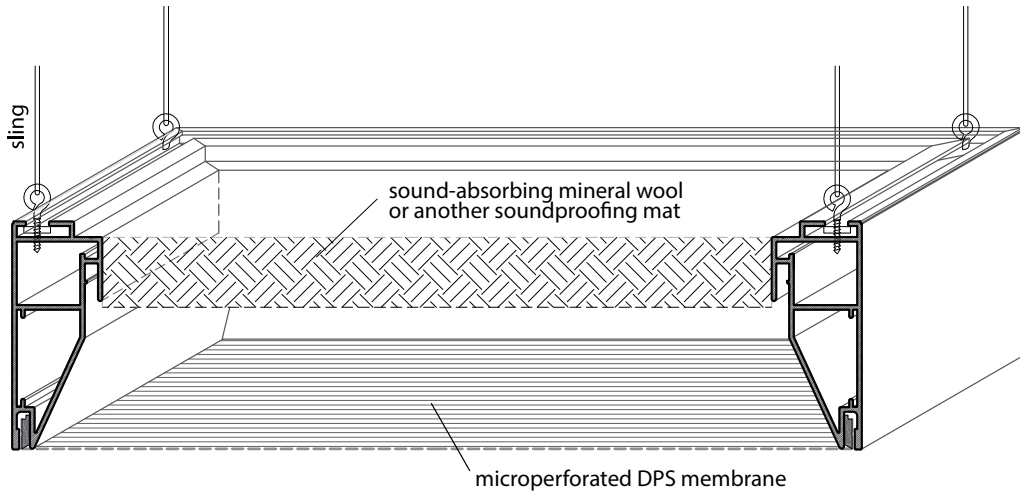
FIG 2. | ACOUSTIC PANEL
