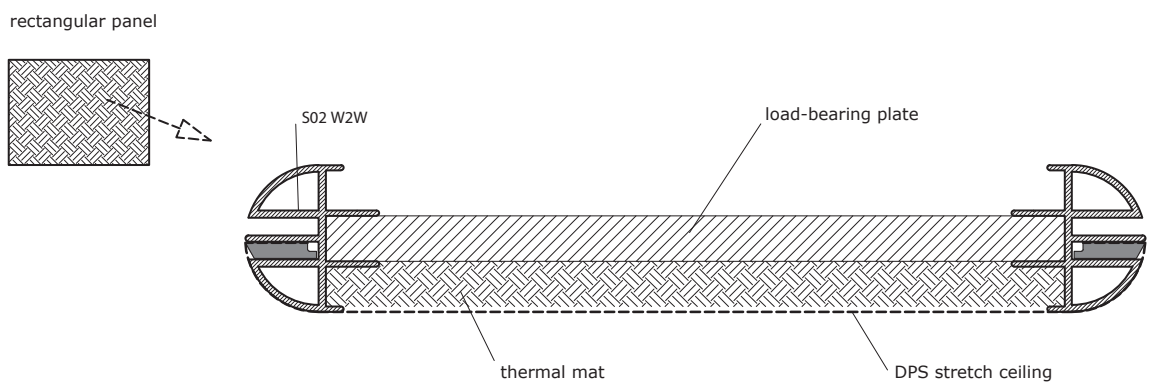
FIG. 4 | THERMAL INSULATION PANEL
