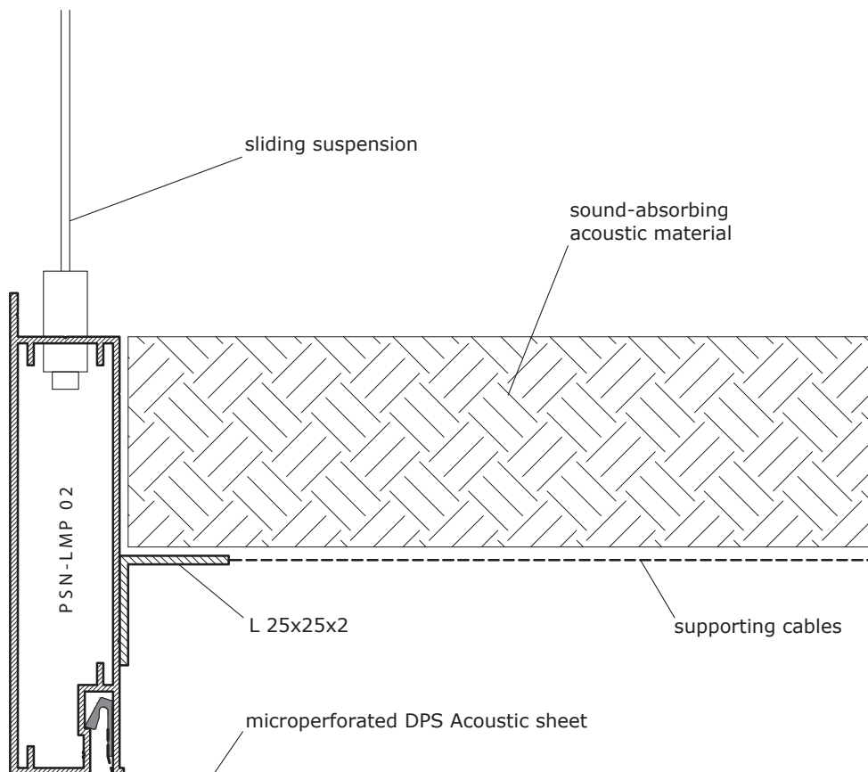
FIG. 3 | ACOUSTIC PANEL
