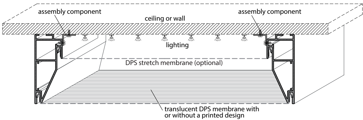
FIG 3. | SEPARATE PANEL - CEILING OR WALL ASSEMBLY
