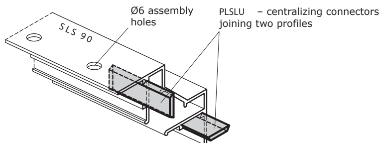
detailed view of two profiles connection
