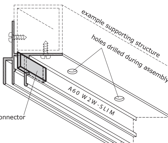
slotless system, W2W harpoon
