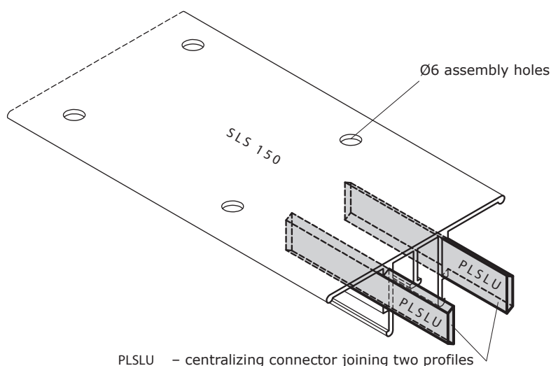
PLSLU – centralizing connector joining two profiles
