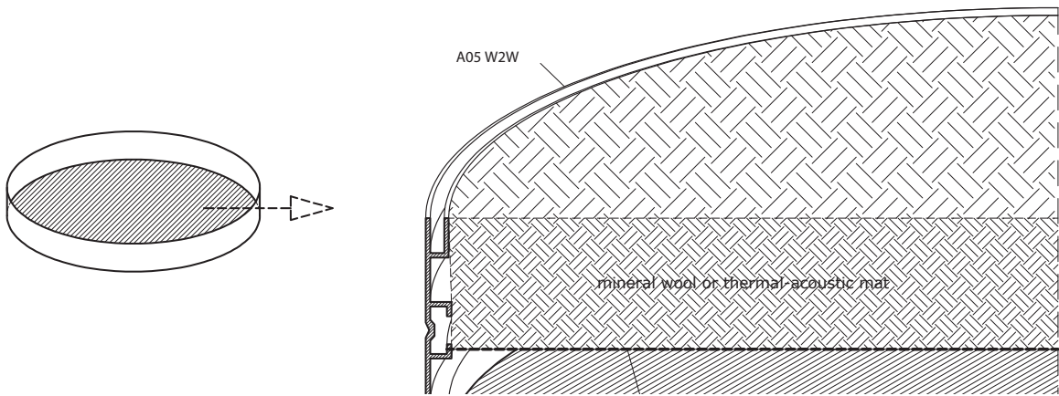
FIG. 2 | ACOUSTIC ELEMENTS
