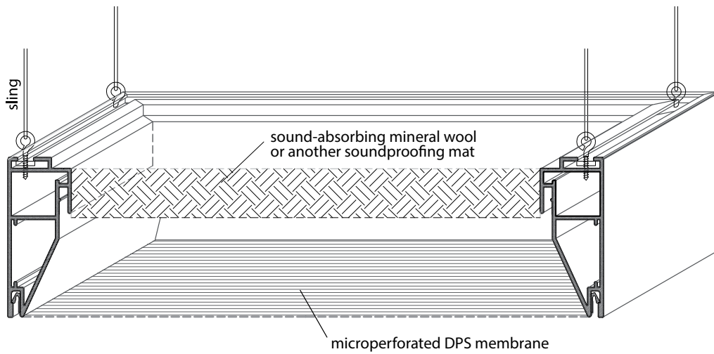
FIG 2. | ACOUSTIC PANEL
